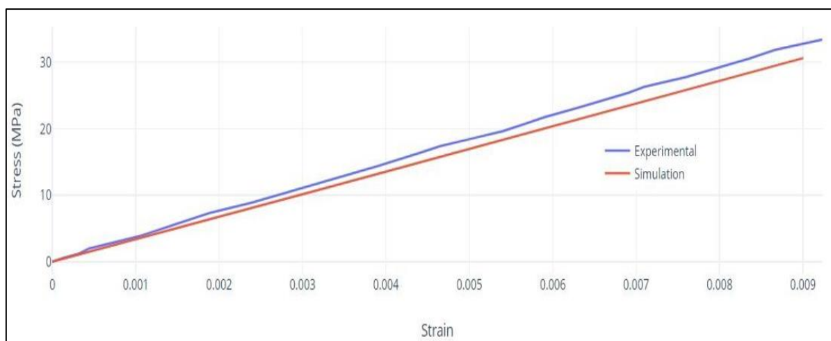
Fig. 13. Graphical comparison for 10mm/s.
