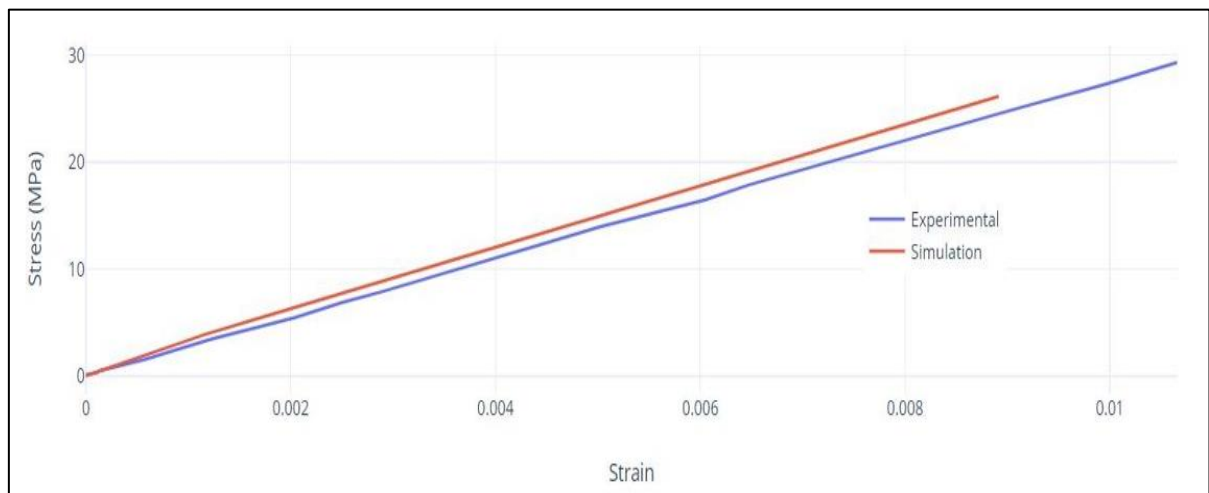
Fig. 12. Graphical comparison for 5mm/s.
