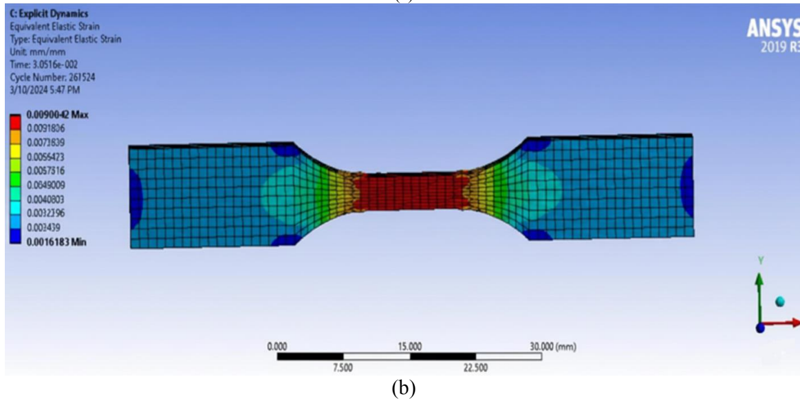
Fig. 9. Simulation output - Equivalent stress and strain at 10 mm/s.
