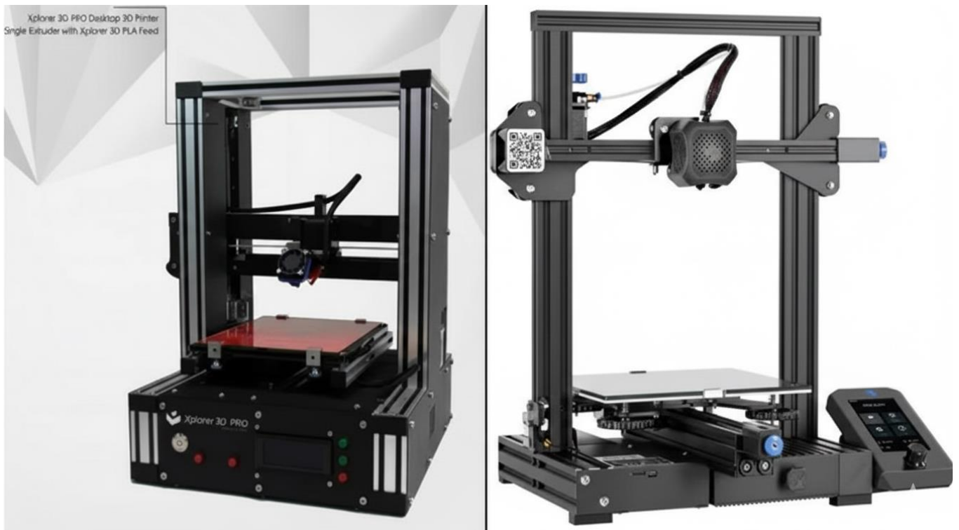
Fig. 2. Xplorer 3D and Ender 3 Pro FDM machines used in this study. The Ender 3 Pro has a build volume of 220 \times 220 \times 250 mm, and the Xplorer 3D machine has a build volume of 200 \times 200 \times 180 mm, which provides dimensional scale for the figure.
