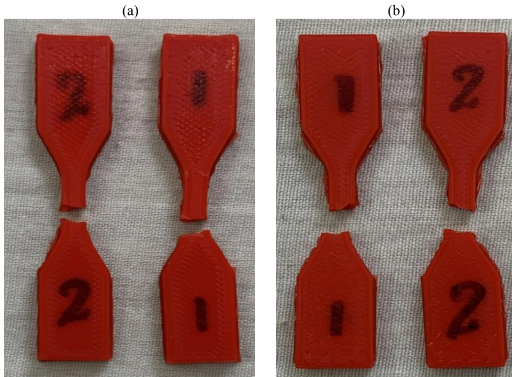
Fig. 16. Printing orientation.
