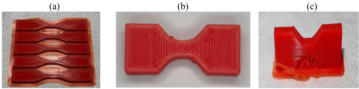
Fig. 5. Live printed ASTM D638 Type-V tensile specimens: (a) 15° raster angle, (b) X-orientation, and (c) on-edge configuration with support structure. Each specimen follows the ASTM D638 Type-V geometry with an overall length of 63.5 mm, gauge length of 7.62 mm, and narrows-section width of 3.18 mm, which provides dimensional scale for the images.
