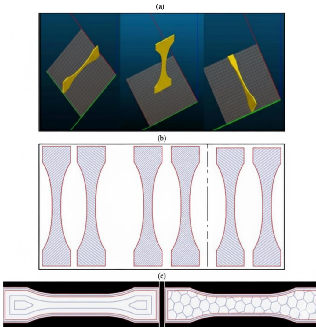
Fig. 4. Printing parameters - (a) Orientations, (b) Raster angles, and (c) Infill patterns.
