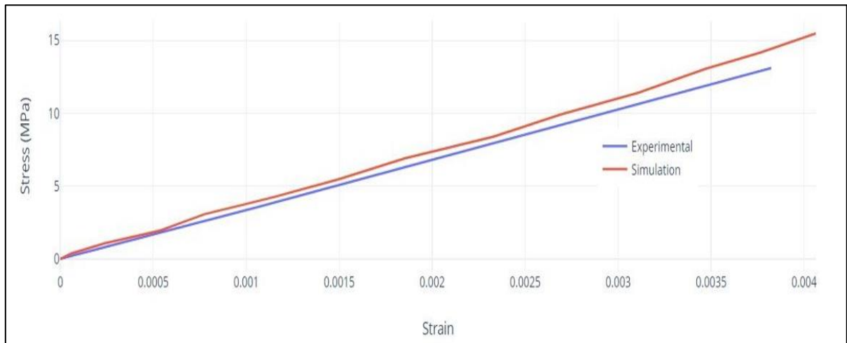
Fig. 11. Graphical comparison for 2mm/s.
