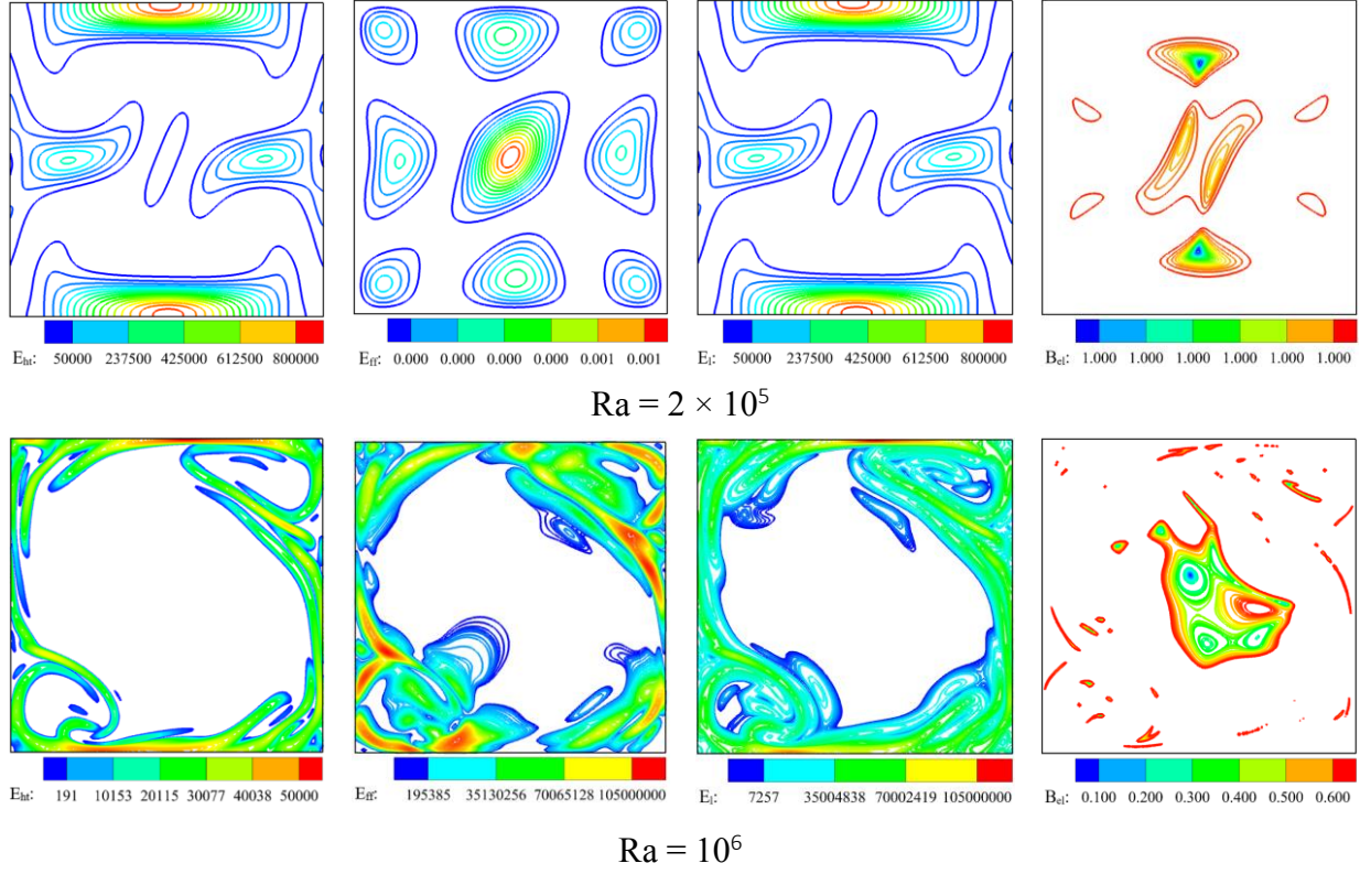
Fig. 9. Distribution of E_{gen} due to HT ( E_{ht} ), E_{gen} due to FF ( E_{ff} ), local E_{gen} ( E_l ), and local B_{el} for the Ra values of 2 \times 10^5 and 10^6 , respectively.
