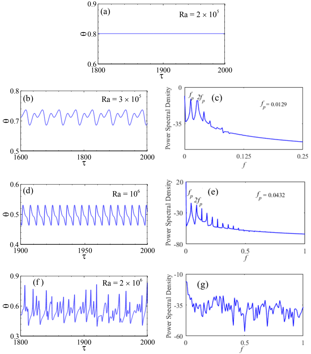
Fig. 7. Temperature time series and the corresponding spectral analysis at point P_3 (0.6, 0.3): (a) steady state for Ra = 2 \times 10^5 ; (b, c) shifting to periodic state for Ra = 3 \times 10^5 ; (d, e) remains periodic for Ra = 10^6 ; and (f, g) changeover to chaotic state for Ra = 2 \times 10^6 .
