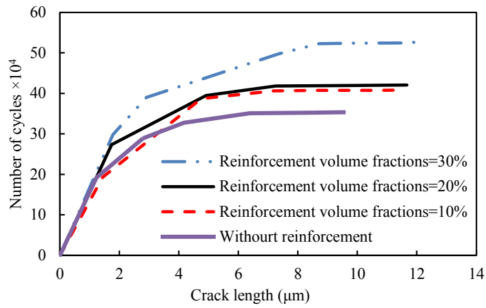
Fig. 27. Effect of triangular particle volume fraction on fatigue life for a constant particle size of 2.66 μm.
