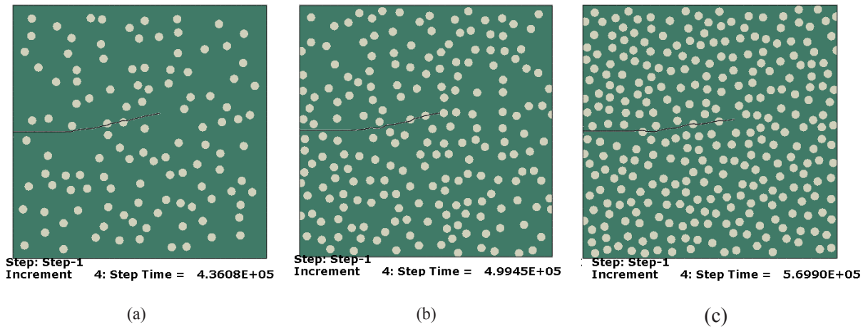
Fig. 15. Distribution of silicon nitride particles and fatigue crack growth path in an FGM plate containing 0.5 μm particles with varying volume fractions a) 10%; b) 20%; c) 30%.
