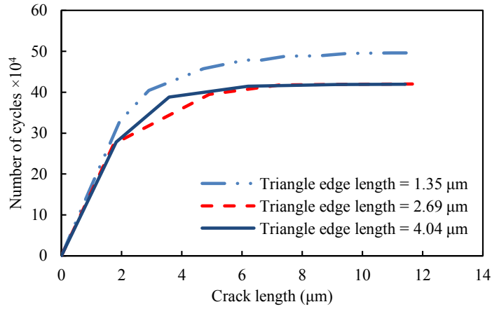
Fig. 24. Effect of triangular particle size on fatigue life of FGM plates with 20% silicon nitride reinforcement.
