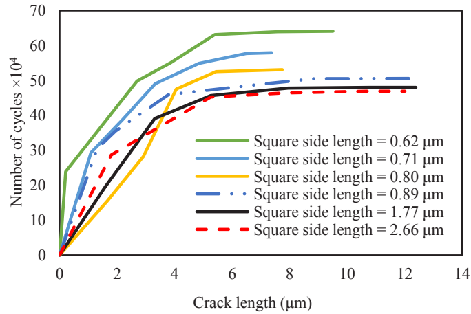
Fig. 33. Effect of square particle size on fatigue life of FGM plates with 20% reinforcement.
