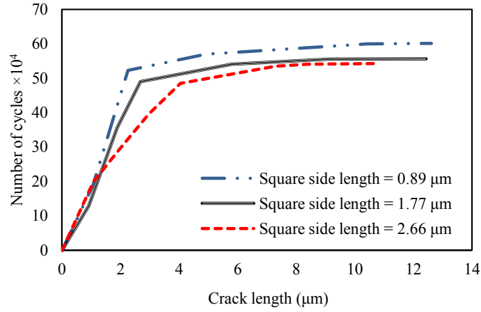
Fig. 11. Effect of square particle size on fatigue life of FGM plates with 30% silicon nitride reinforcement.
