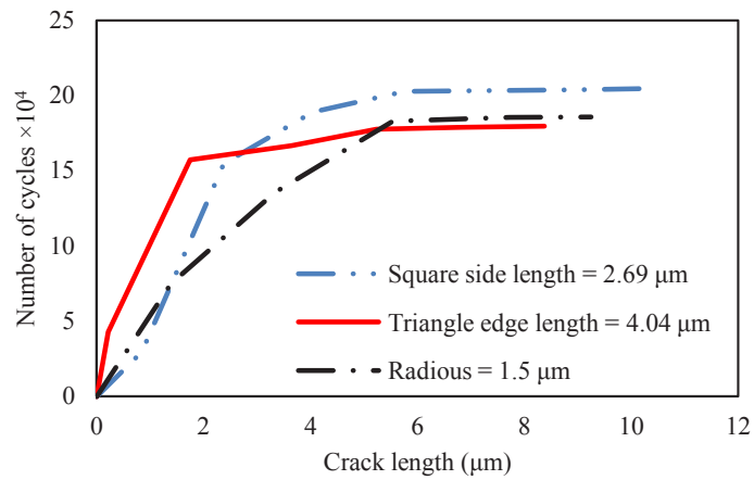
Fig. 31. Effect of particles shape on FGM fatigue life at 30% volume fraction under mixed-mode loading conditions.
