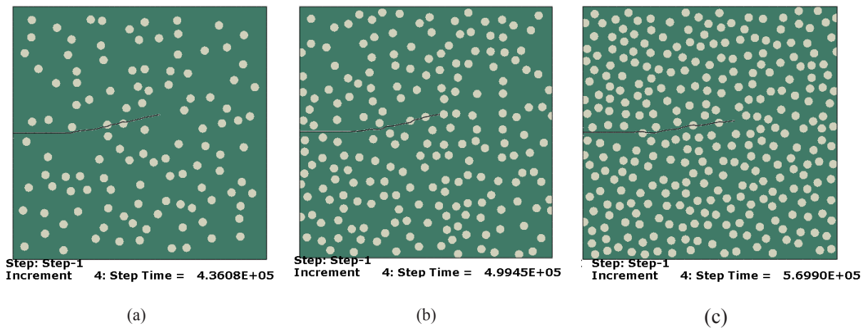
Fig. 15. Distribution of silicon nitride particles and fatigue crack growth path in an FGM plate containing 0.5 μm particles with varying volume fractions a) 10%; b) 20%; c) 30%.
