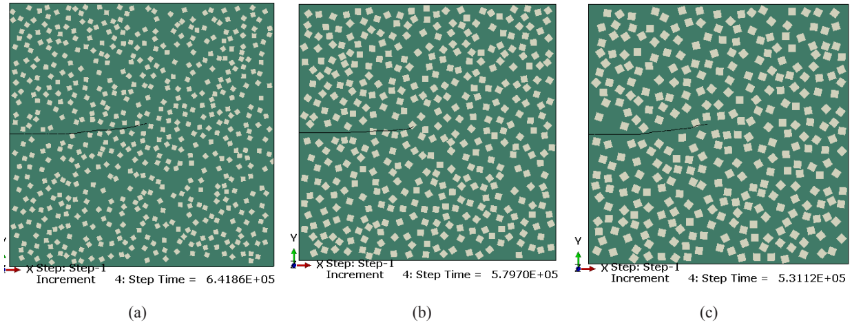
Fig. 32. Distribution of silicon nitride particles and fatigue crack growth path in an FGM plate containing 20% particles with varying square side length a) 0.62 \mu\text{m} ; b) 0.71 \mu\text{m} ; c) 0.80 \mu\text{m} .
