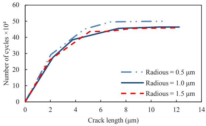
Fig. 17. Effect of circular particle size on fatigue life of FGM plates with 20% silicon nitride reinforcement.
