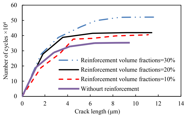
Fig. 28. Effect of triangular particle volume fraction on fatigue life for a constant particle size of 4.04 μm.
