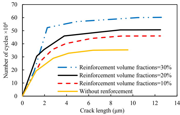
Fig. 12. Effect of square silicon nitride particle volume fraction on fatigue life for a constant particle size of 0.89 μm.
