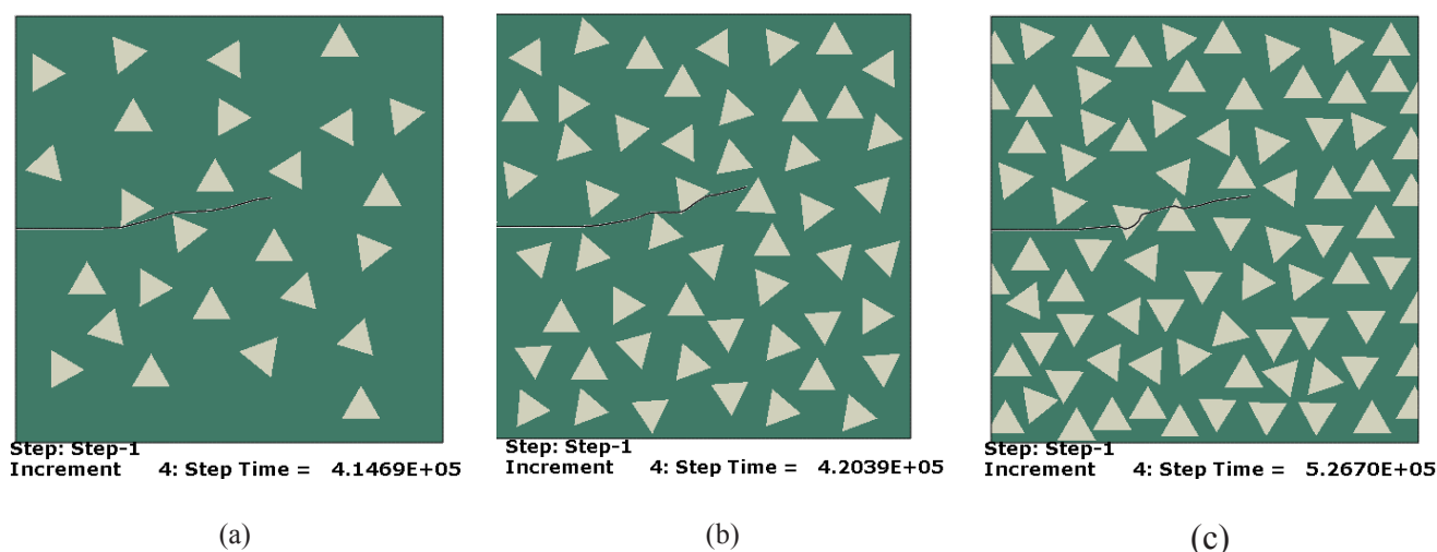
Fig. 22. Distribution of triangular silicon nitride particles and fatigue crack growth path in an FGM plate containing 2.66 \mu\text{m} particles with varying volume fractions a) 10%; b) 20%; c) 30%.
