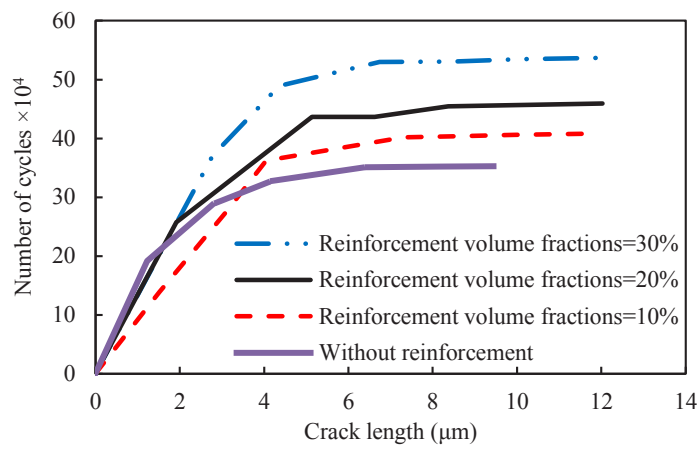
Fig. 21. Effect of circular particles volume fraction on fatigue life for a constant particle size of 1.5 μm.
