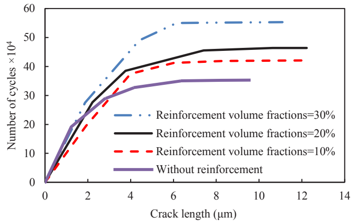
Fig. 20. Effect of circular particles volume fraction on fatigue life for a constant particle size of 1 μm
