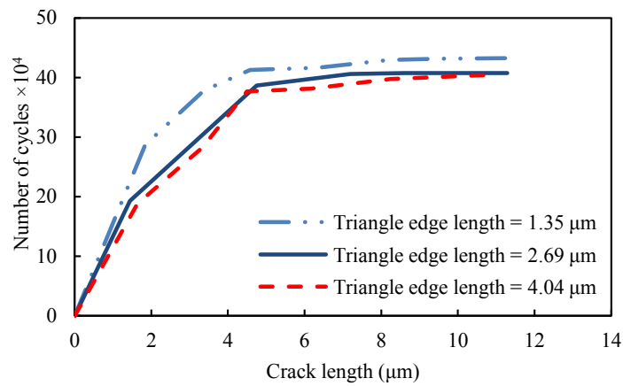
Fig. 25. Effect of triangular particle size on fatigue life of FGM plates with 30% silicon nitride reinforcement.
