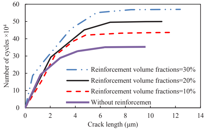
Fig. 19. Effect of circular particles volume fraction on fatigue life for a constant particle size of 0.5 μm.
