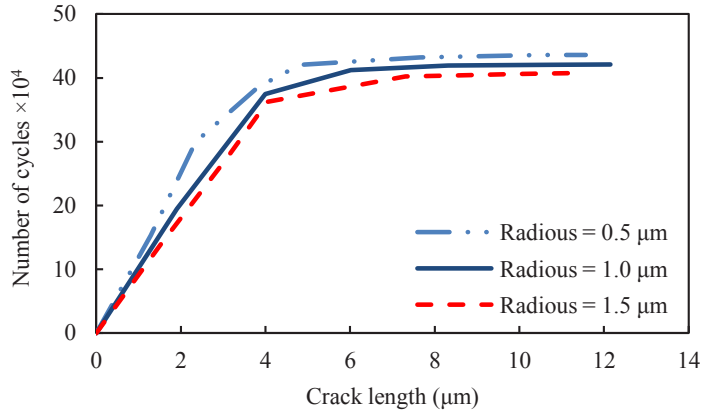
Fig. 16. Effect of circular particle size on fatigue life of FGM plates with 10% silicon nitride reinforcement.
