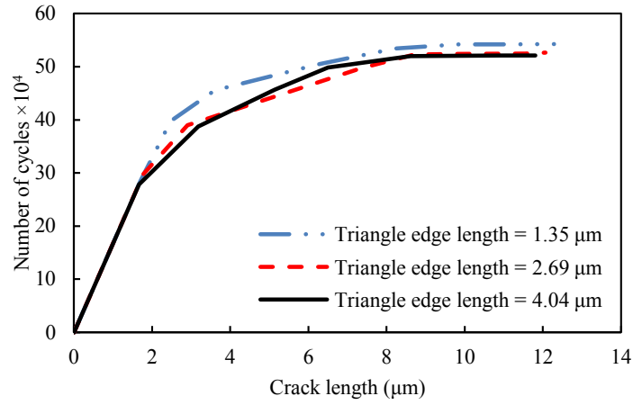
Fig. 23. Effect of triangular particle size on fatigue life of FGM plates with 10% silicon nitride reinforcement.
