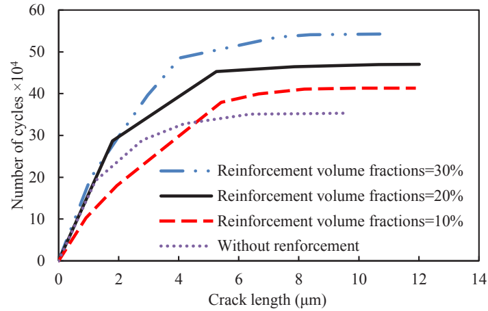
Fig. 14. Effect of square silicon nitride particle volume fraction on fatigue life for a constant particle size of 2.66 μm.
