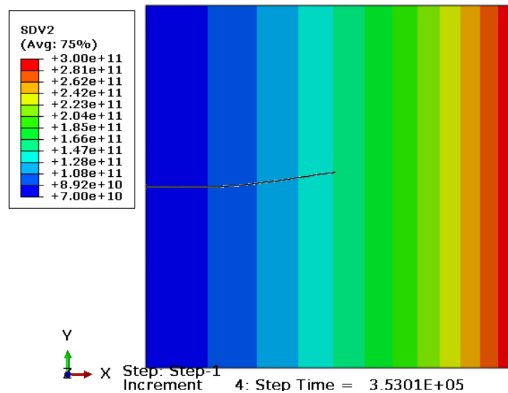
Fig. 6. Crack growth in an FGM plate.
