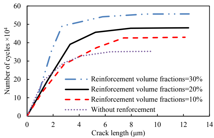
Fig. 13. Effect of square silicon nitride particle volume fraction on fatigue life for a constant particle size of 1.77 μm.
