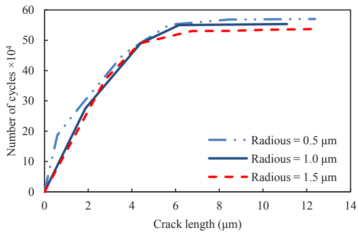
Fig. 18. Effect of circular particle size on fatigue life of FGM Plates with 30% silicon nitride reinforcement.
