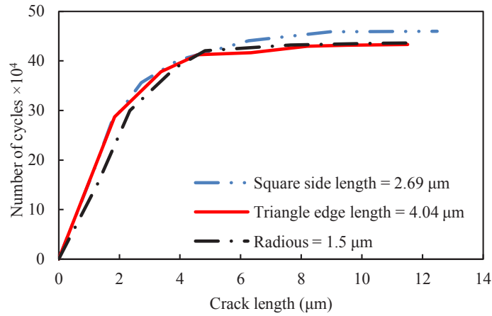
Fig. 30. Comparative study of various particle shapes in FGM fatigue life at 30% volume fraction.
