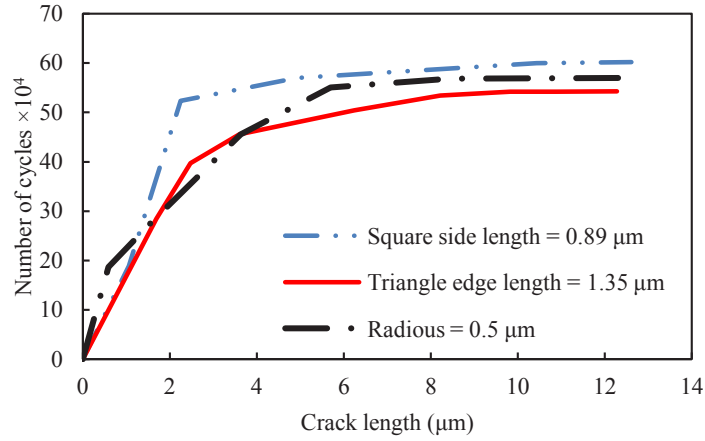
Fig. 29. Effect of particles shape on FGM fatigue life at 30% volume fraction.
