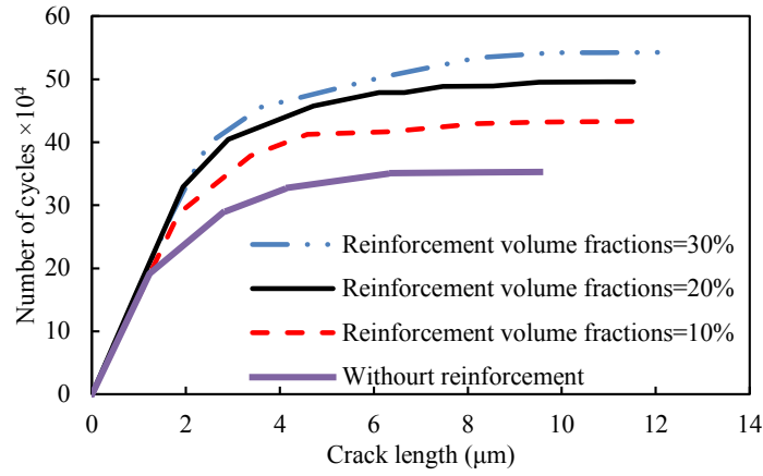
Fig. 26. Effect of triangular particle volume fraction on fatigue life for a constant particle size of 1.35 μm.
