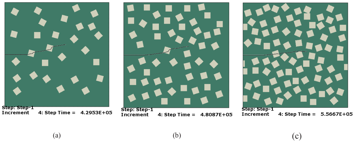
Fig. 8. Distribution of silicon nitride particles and fatigue crack growth path in an FGM plate containing 1.77 \mu\text{m} side length particles with varying volume fractions a) 10%; b) 20%; c) 30%.
