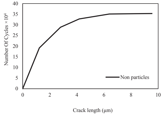
Fig. 5. Fatigue crack growth rate versus cycles to failure.
