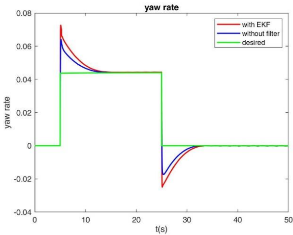
c. yaw rate
