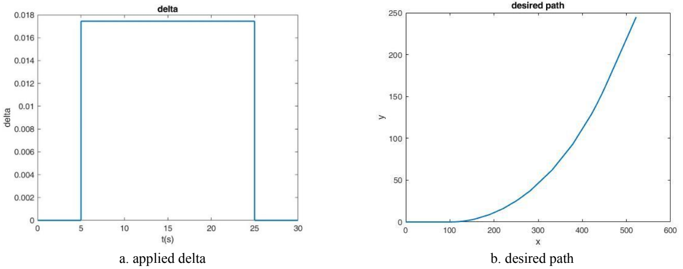
Fig. 6. Desired maneuver applied on vehicle
