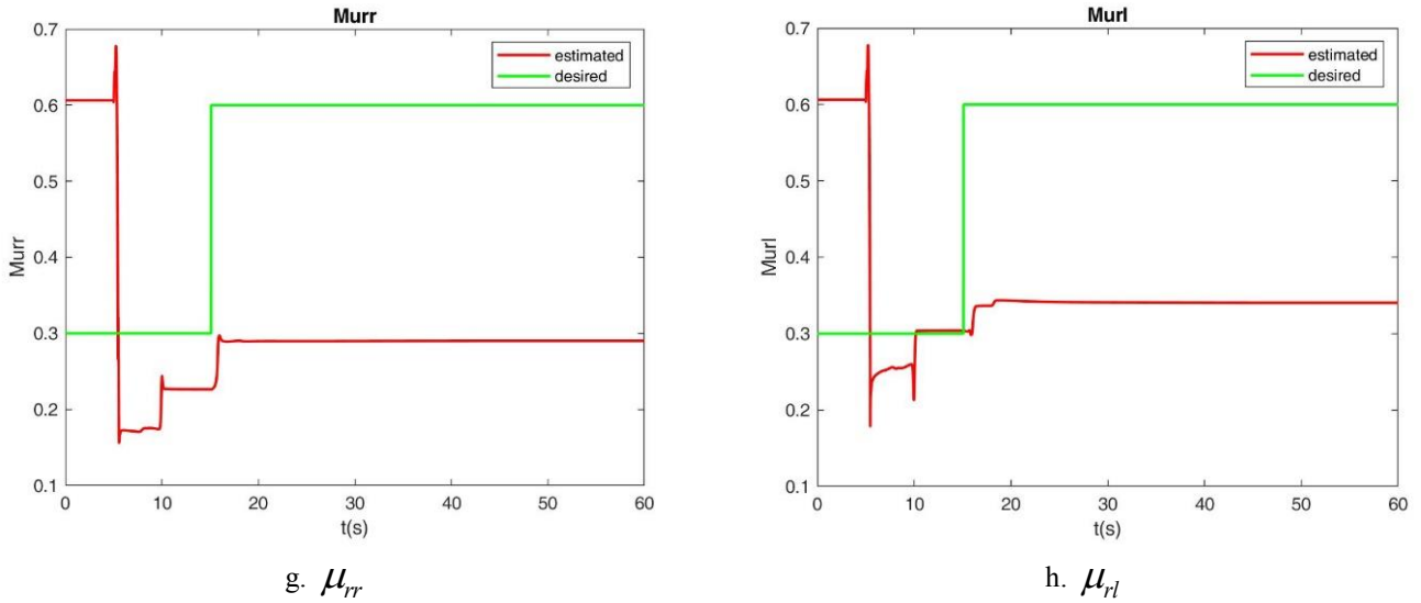
Fig. 14. The process of estimating the friction coefficient of wheels with EKF where the desired friction coefficient was changed
