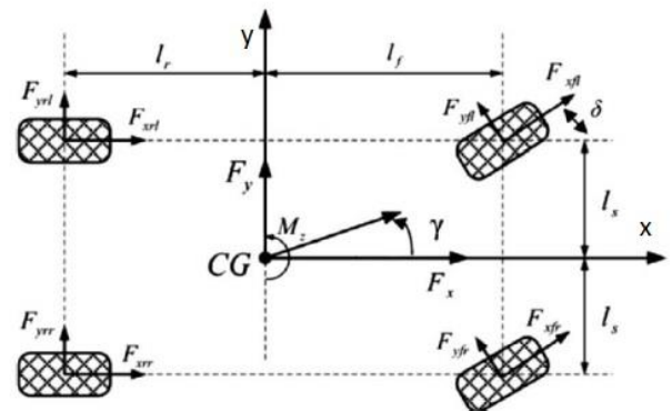
Fig. 1. Four-wheel vehicle model [22]
