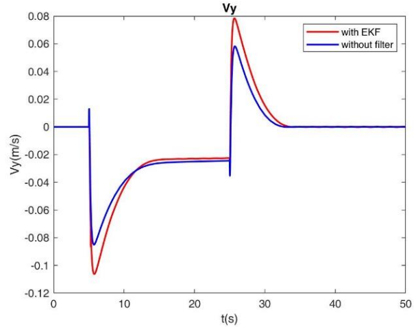
b. lateral speed
