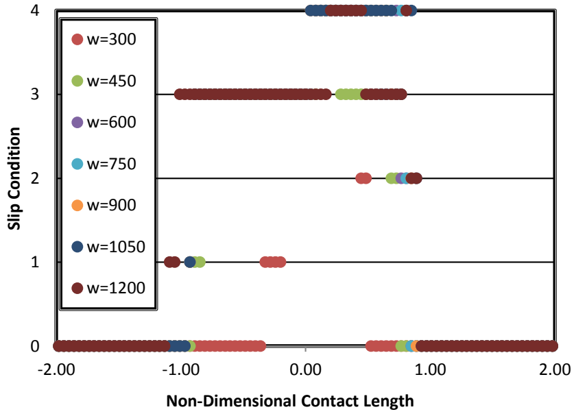
Fig. 6. The range and the condition of slips occurred for different loads
