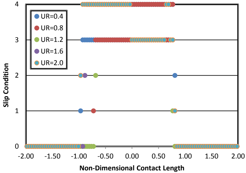
Fig. 7. The range and the condition of slips occurred for different velocity ratios
