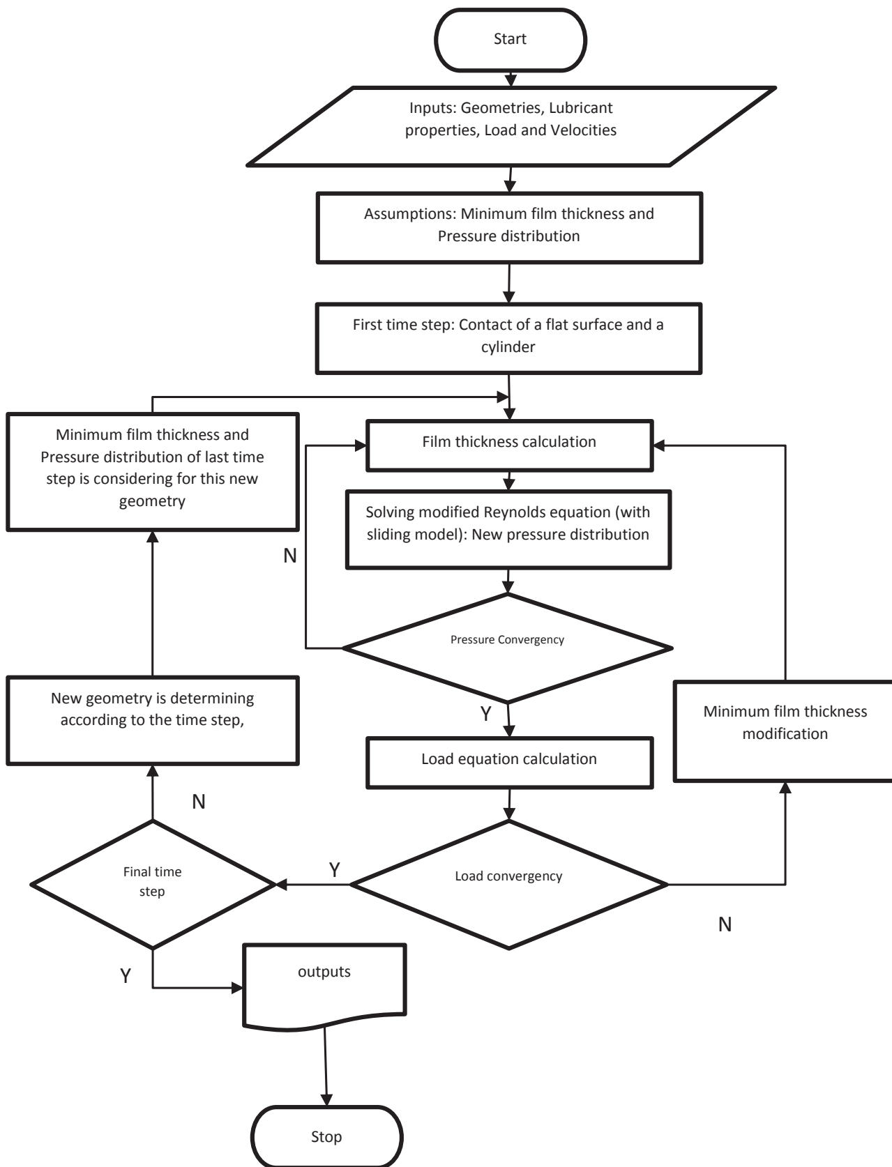
Fig. 3. The elastohydrodynamic problem-solving algorithm
