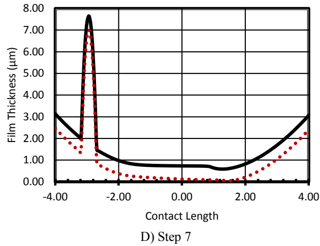
Fig. 5. Lubricant film thickness distribution over contact length for various time steps with slip and no-slip condition. —— : Slip condition ●●● : No-slip condition
