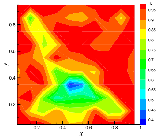
Fig. 6. Inverse reconstruction of the K -distribution in an absorbing-emitting medium with a low absorption coefficient at the first step
