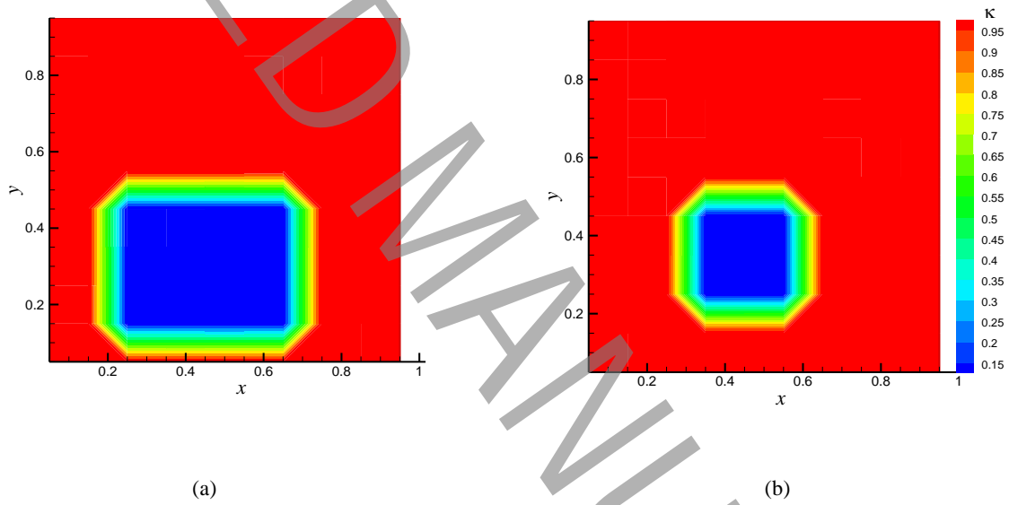
Figs.7. K -distribution (a) initial guess, and (b) inverse reconstruction in an absorbing-emitting medium with a low absorption coefficient at the second step
