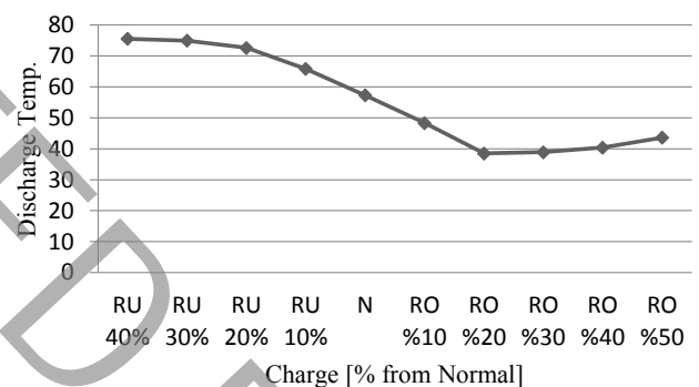
Fig. 4. The effect of refrigerant charge on compressor discharge temperature (°C).
